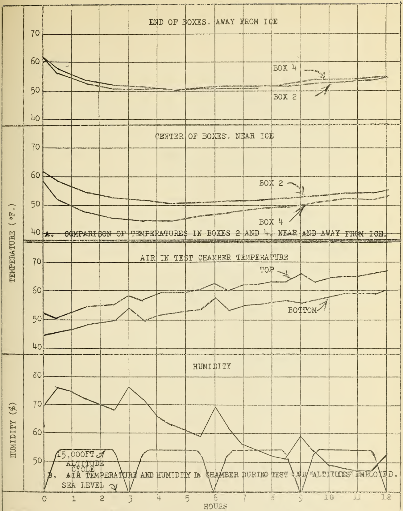
Fig. 9 FLOWER TEMPERATURE IN TWO "SMALL" 2 1/2 INCH BOXES. TEST 9. 6 BOX 2 WITH 5 POUNDS OF ICE AND WET PAPER (A 1/2 LB. P.C.). BOX 4 WITH 5 POUNDS OF ICE IN MOISTUREPROOF PAPER AND ONE POUND OF DRY ICE OUTSIDE THE BAG (A DRY PACK).
